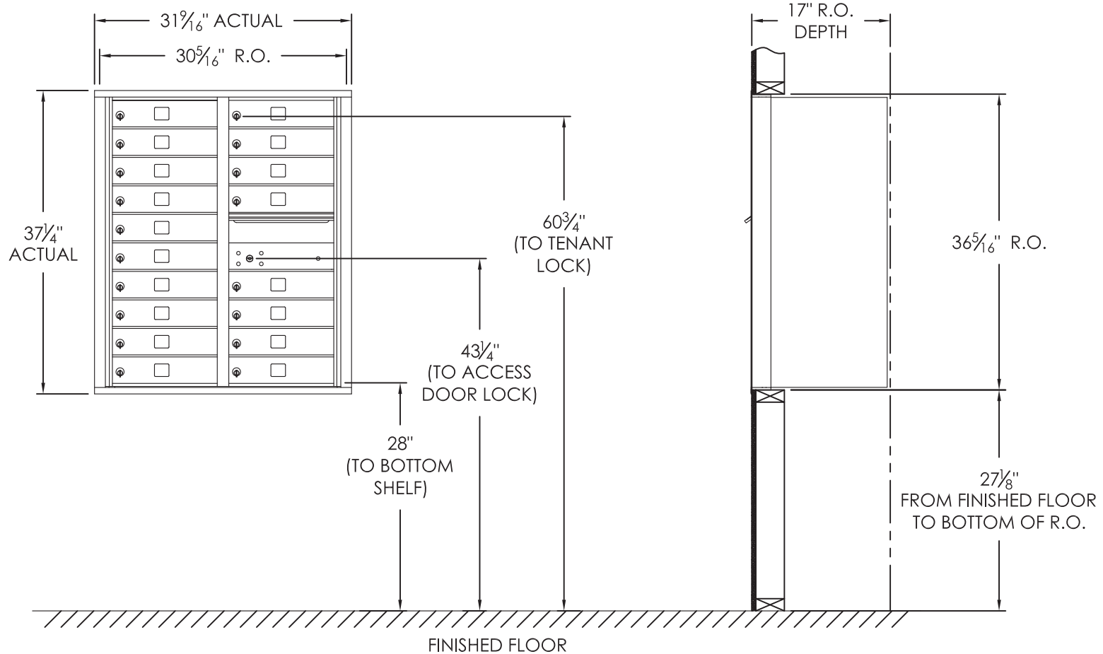
COMPARTMENT CHART
