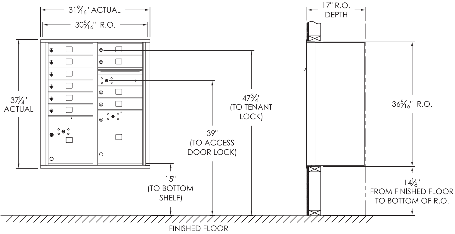
COMPARTMENT CHART
