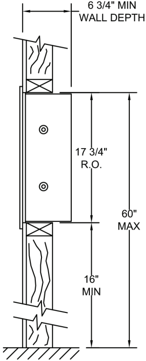
FINISHED FLOOR (RECESS MOUNT)
